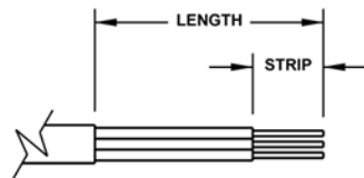
CORDAGE PREPARATION
